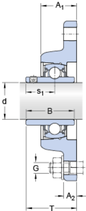
FYT 45 TF/VA228 Bearing 2D drawings and 3D CAD models
